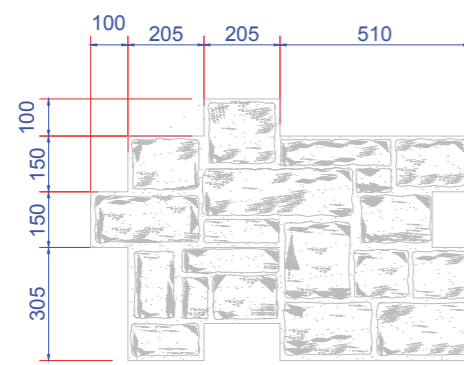
Large Antica Cobble
