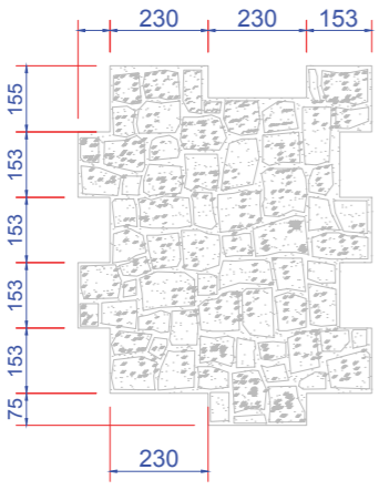
Tumbled Granite Rubble
