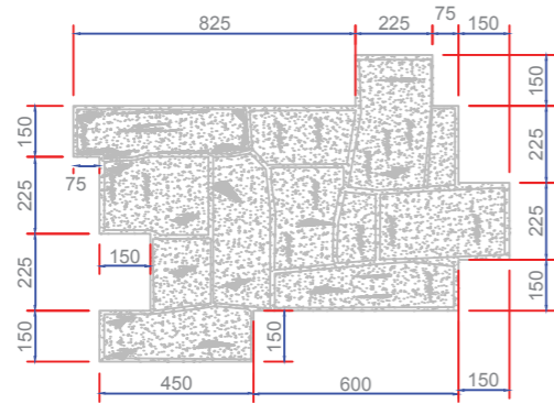
Crazy Cut Italian Slate
